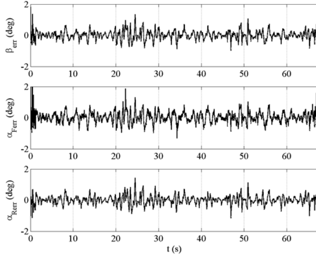
Figure 7 experimental measurement noise
