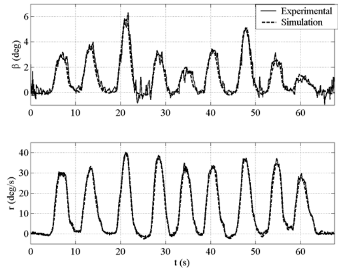
Figure 4 comparison of yaw rate and slip angle
