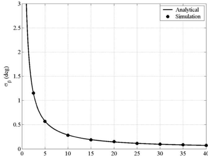
Figure 6 slip angle accuracy
