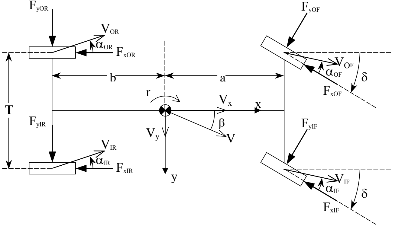
Figure 1 model of system
