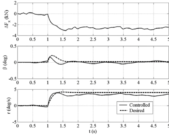
Figure 11 controlled braking system response
