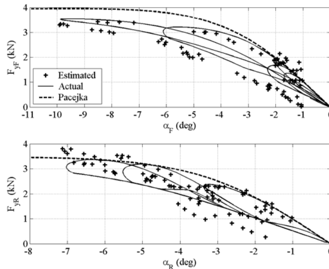
Figure 12 predicted tire curves
