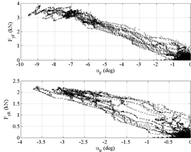
Figure 13 experimental tire curves
