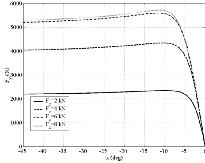
Figure 2 Pacejka tire model for various loading cases
