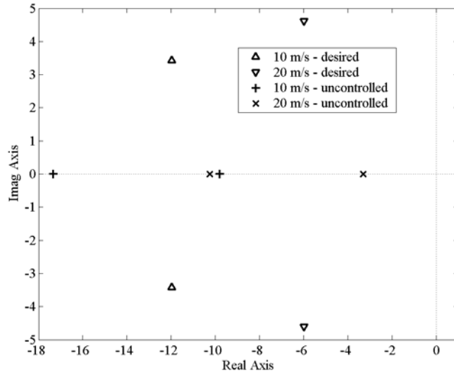
Figure 8 poles of desired and uncontrolled system
