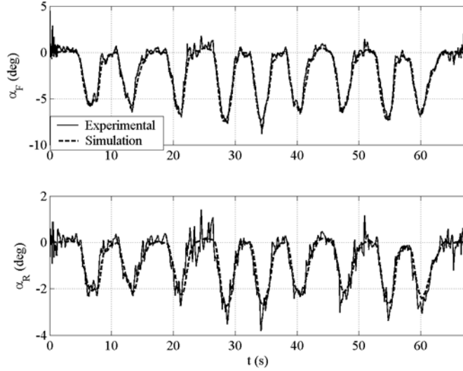
Figure 5 comparison of tire slip angles
