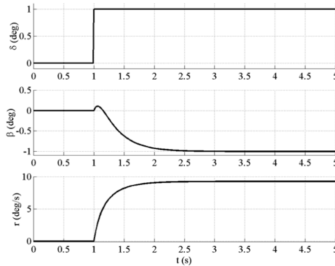
Figure 9 uncontrolled system response
