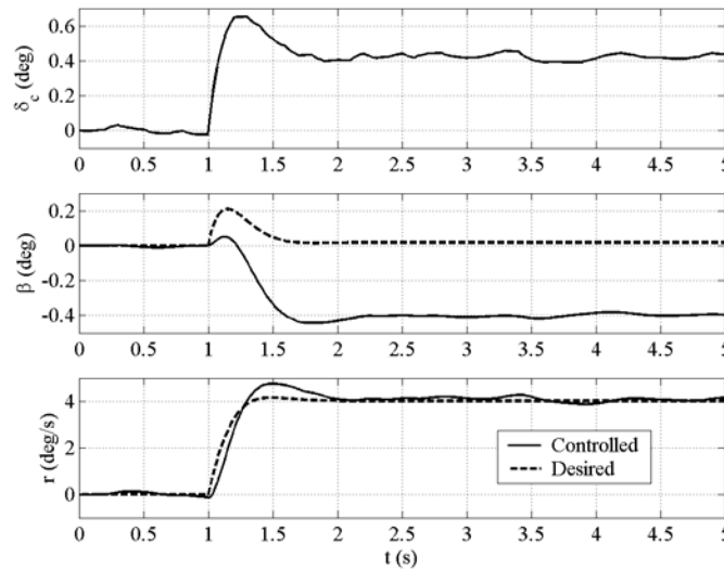
Figure 10 controlled steering system response
